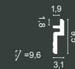
C394 STEPS 200 x 9,5 x 3,1 cm Purotouch® Designed by Orio Tonini
