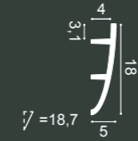
C374 ANTONIO 200 x 18 x 5 cm Purotouch® Designed by Ulf Moritz
