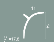
C991 200 x 14 x 11 cm Purotouch® Designed by Ulf Moritz
